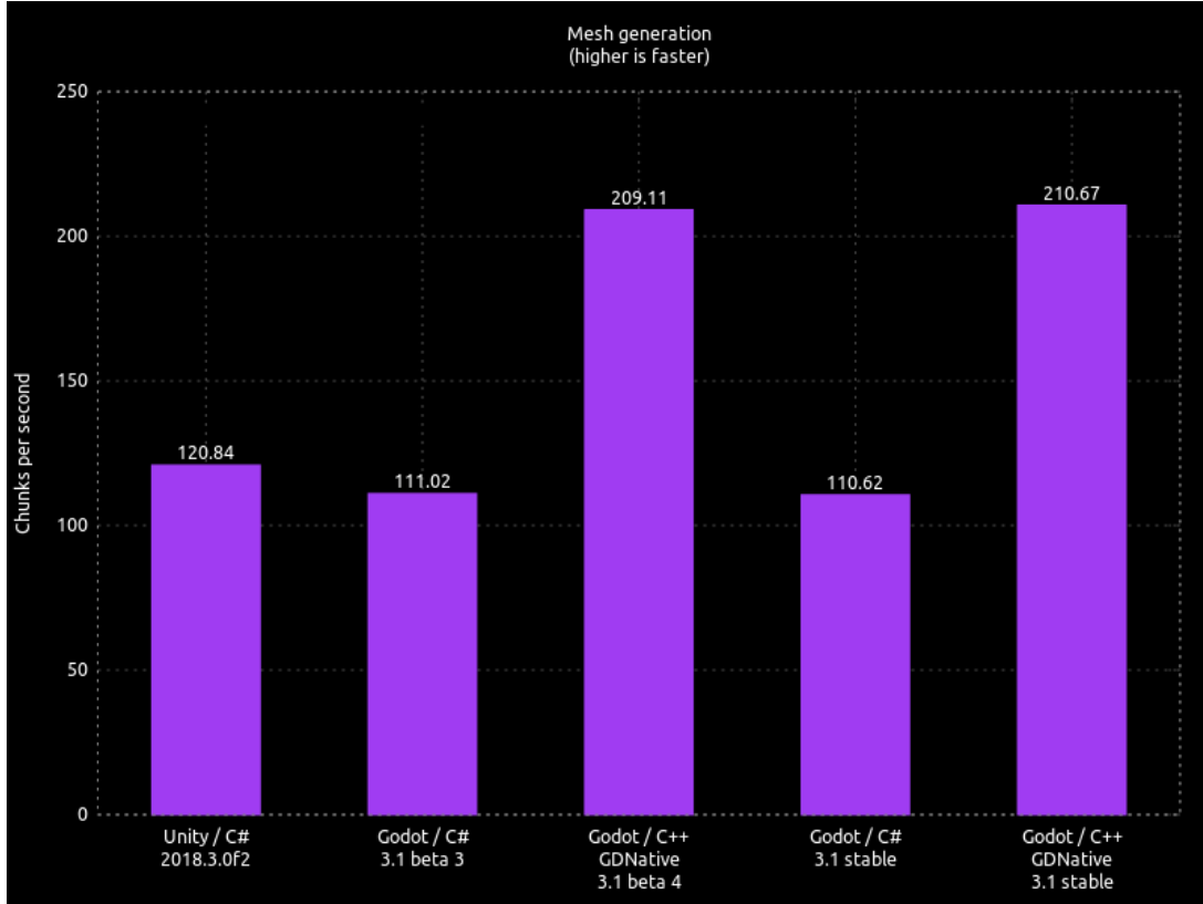
Figura 3: Mesh Generation [6]
